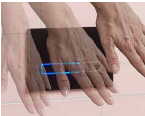
Contactless sensor flush plate 210(w) x 142(h) x 113(d)mm
